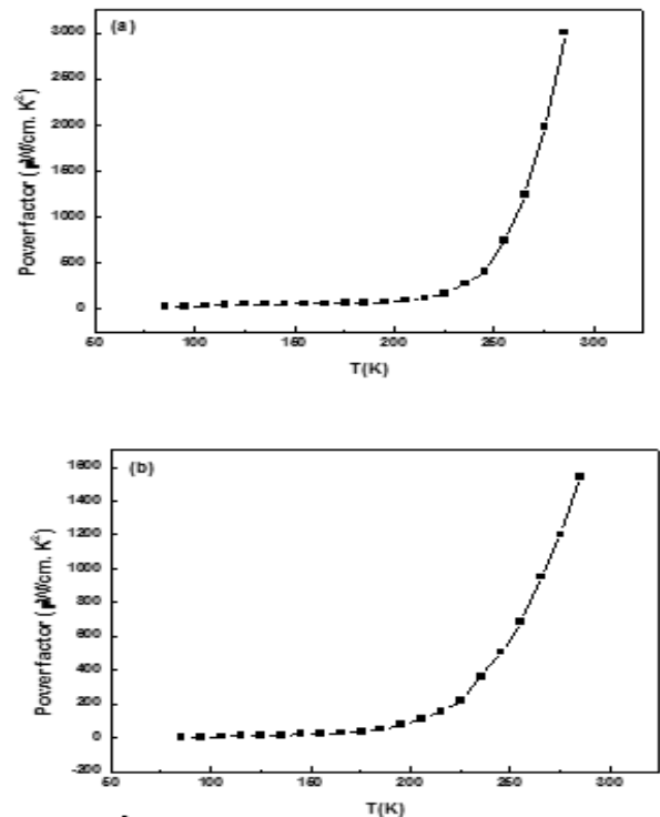
Figure (9): The power factor S^2/\rho plotted as a function of the temperature of as prepared a- NSMOC1 and b-NSMOC2 samples.
